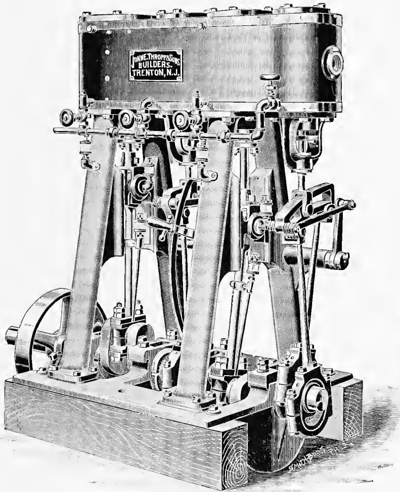
THROPP'S COMPOUND MARINE ENGINE.—Built by John E. Thropp & Sons.
